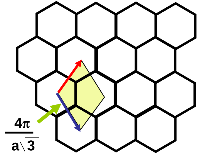
Reciprocal space
