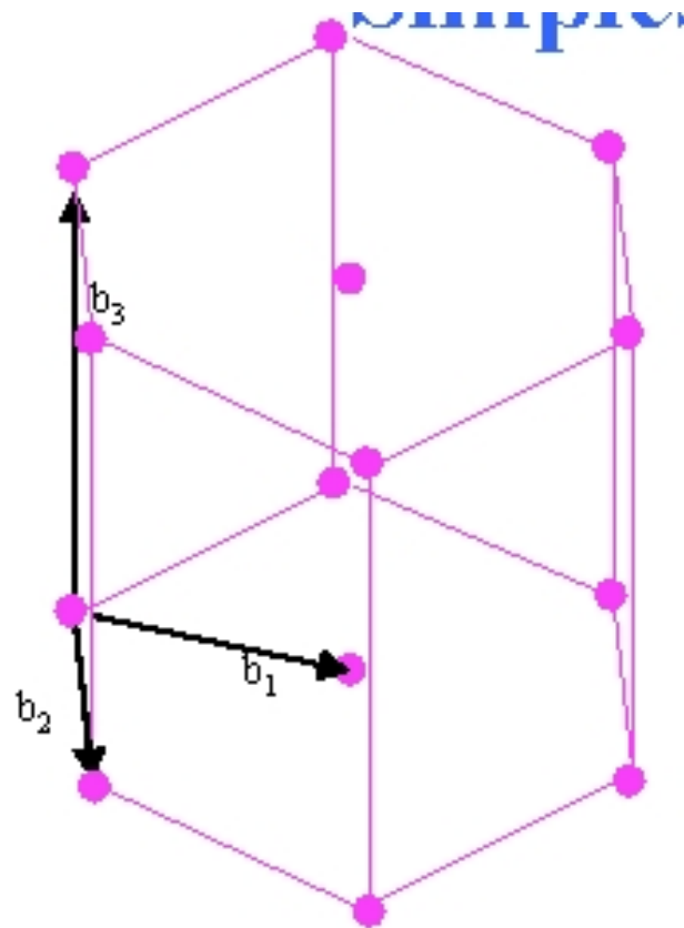
Reciprocal Lattice
